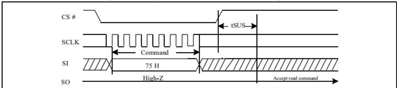
Figure 30. Program/Erase Suspend Sequence Diagram
