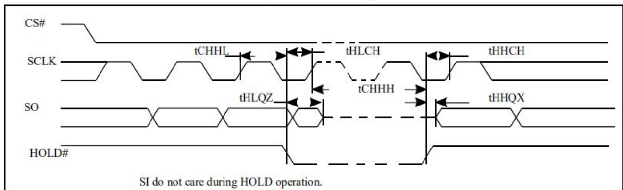
Figure43. Hold Timing
