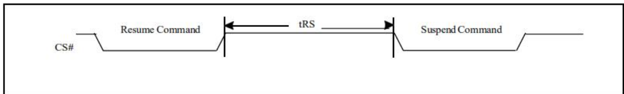
Figure 42. Resume to Suspend Timing Diagram
