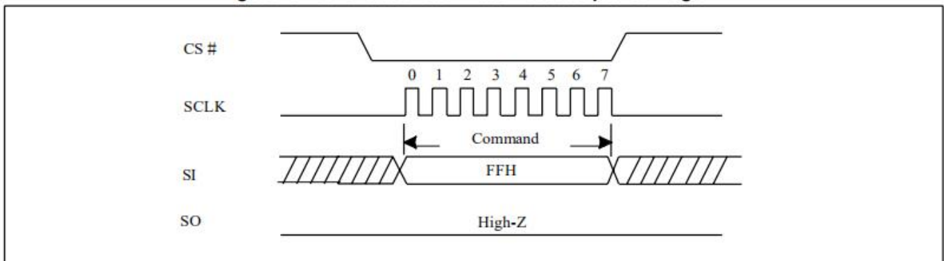
Figure 28. Continuous Read Mode Reset Sequence Diagram
