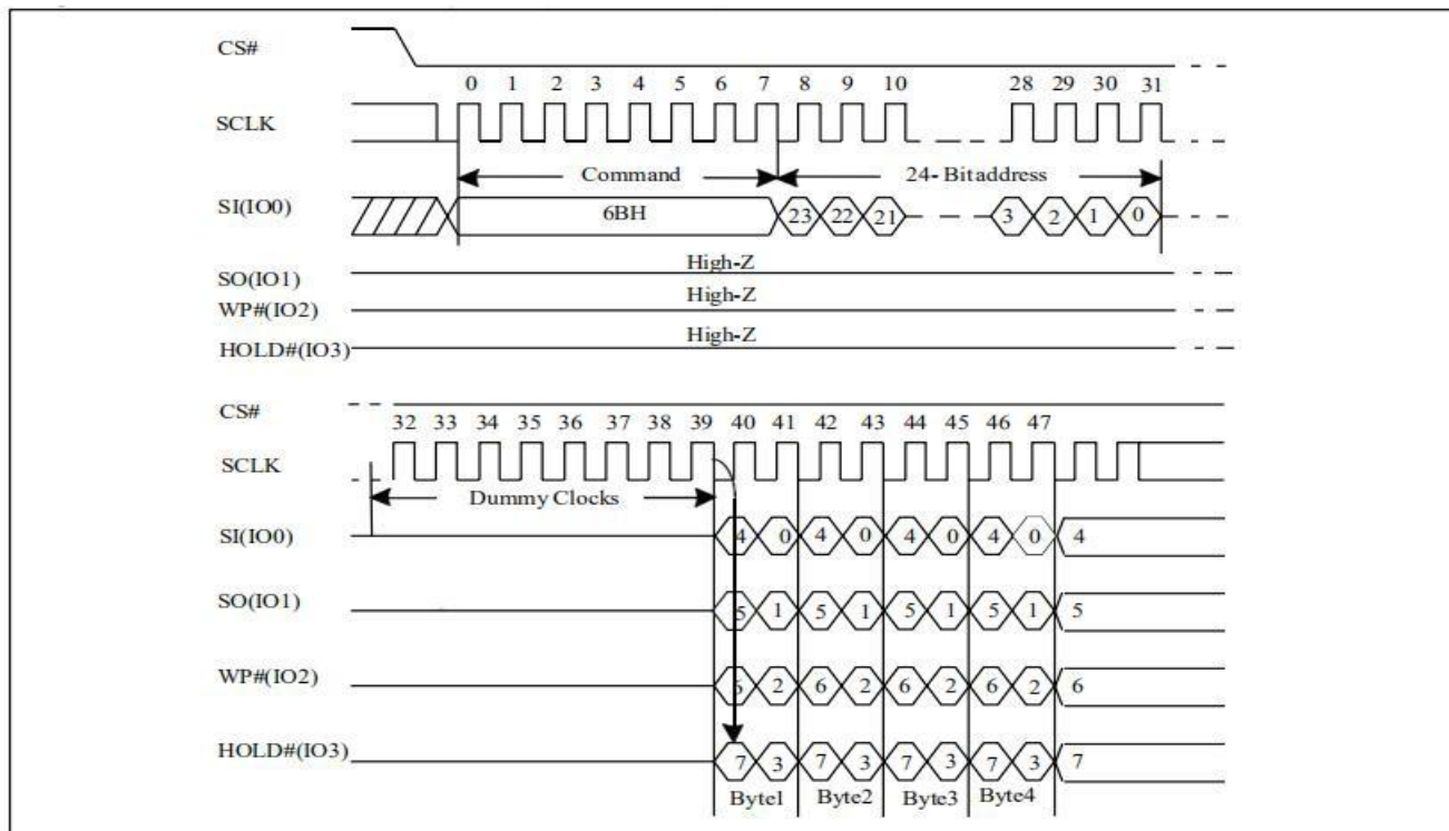
Figure10. Quad Output Fast Read Sequence Diagram
