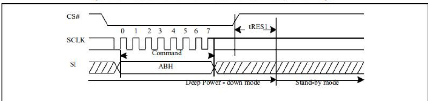
Figure 25. Release Power-Down/Read Device ID Sequence Diagram
