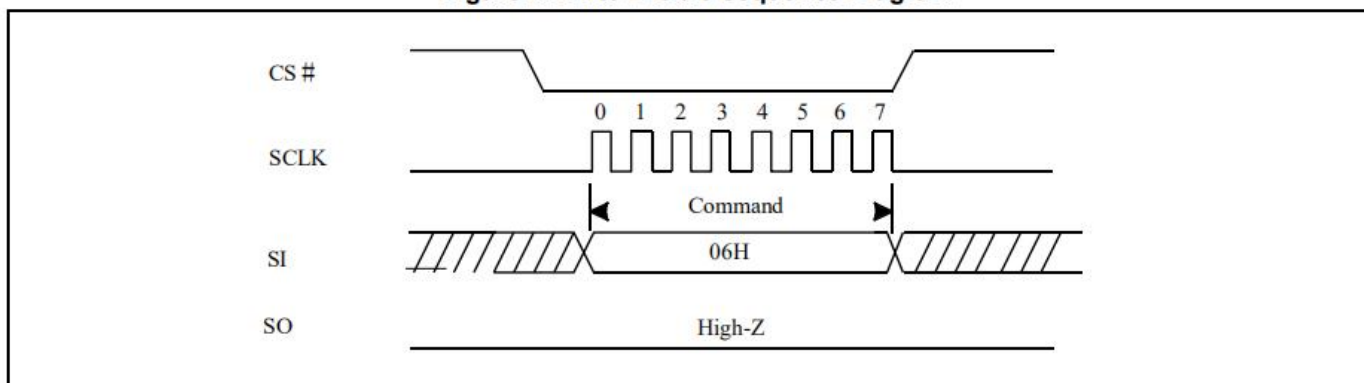
Figure 2. Write Enable Sequence Diagram
