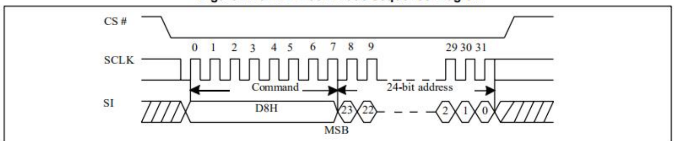
Figure21. 64KB Block Erase Sequence Diagram
