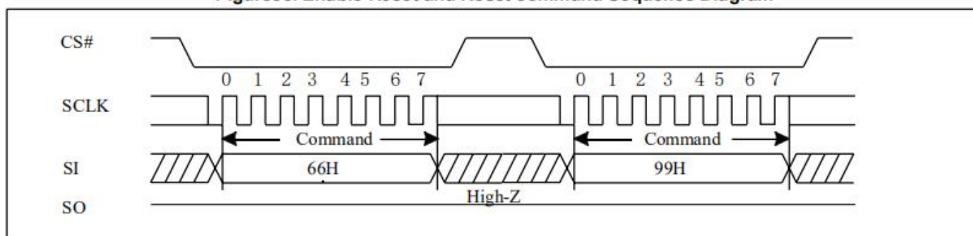
Figure35. Enable Reset and Reset command Sequence Diagram
