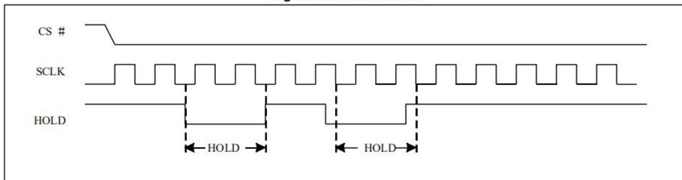
Figure 1. Hold Condition
