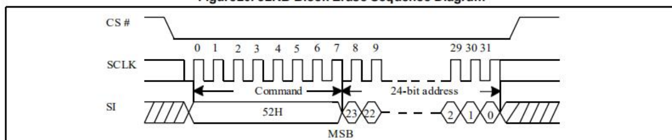
Figure20. 32KB Block Erase Sequence Diagram
