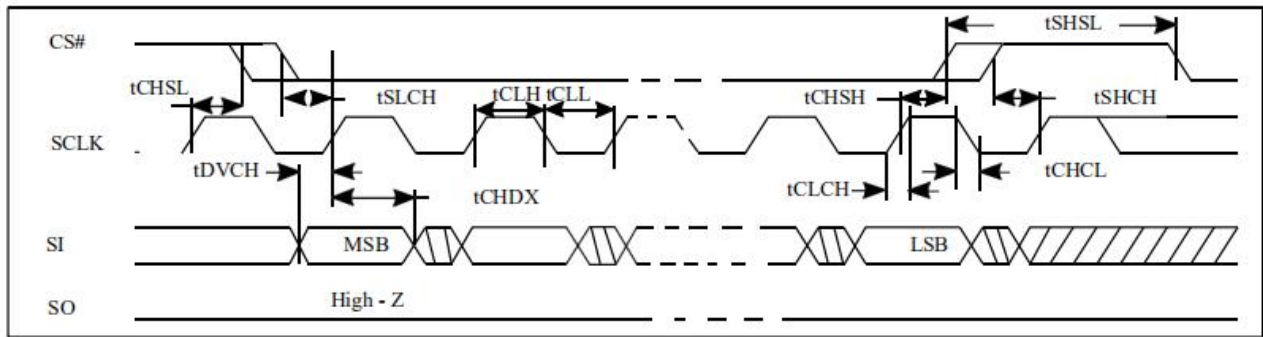
Figure41. Output Timing
