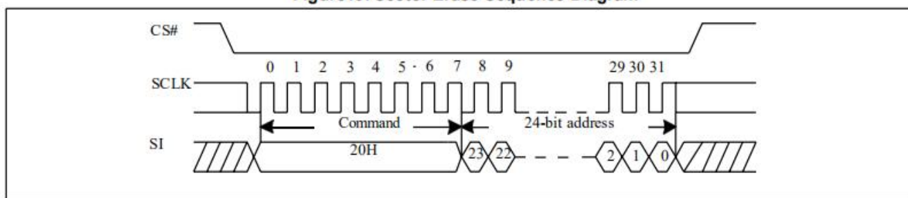
Figure19. Sector Erase Sequence Diagram
