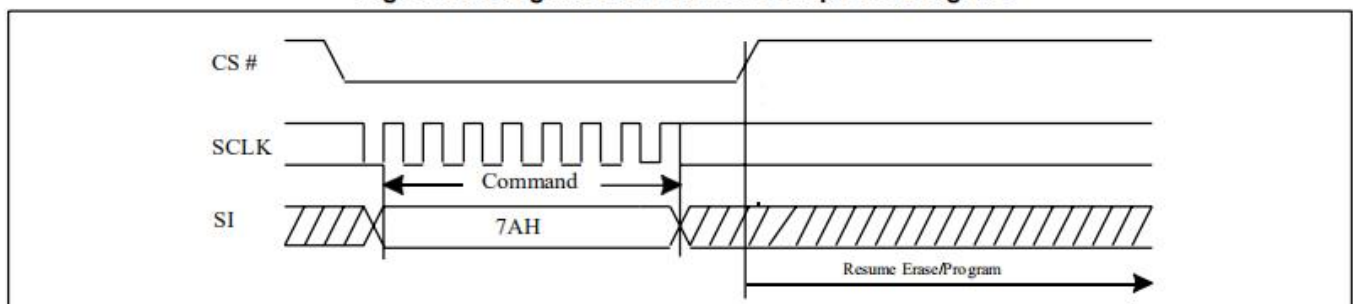
Figure 31. Program/Erase Resume Sequence Diagram
