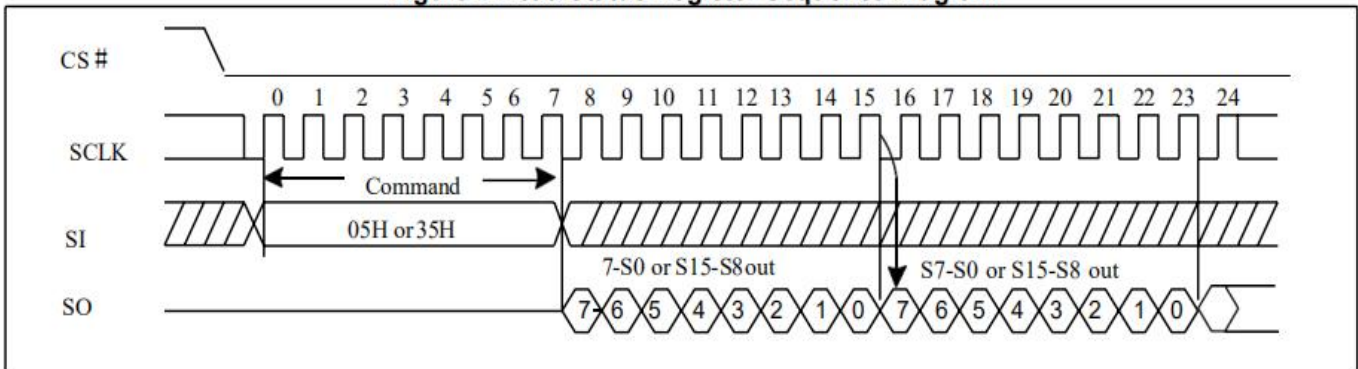
Figure4. Read Status Register Sequence Diagram
