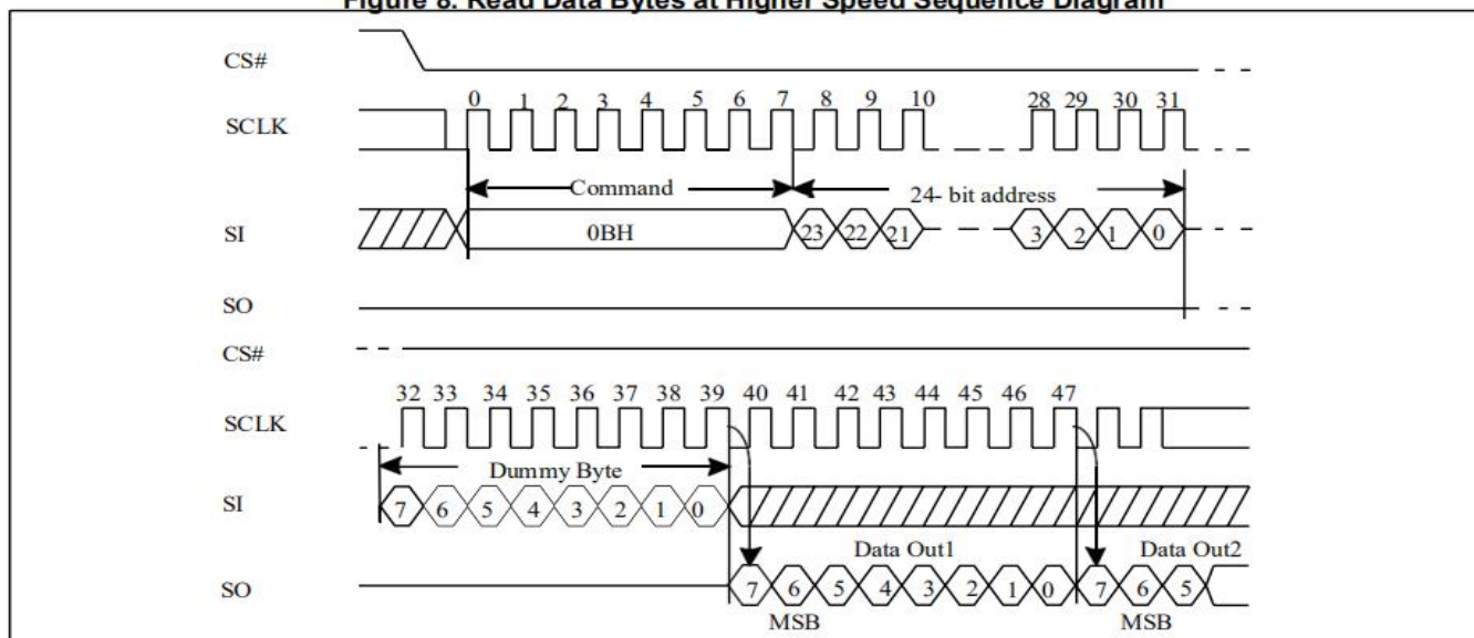
Figure 8. Read Data Bytes at Higher Speed Sequence Diagram
