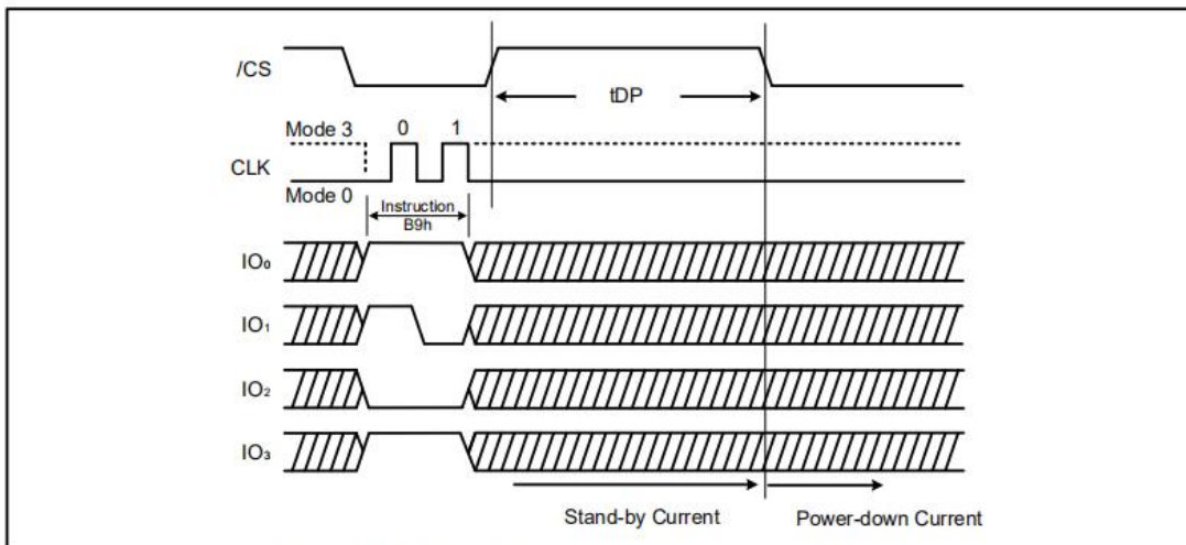
Figure 26b. Deep Power-down Instruction (QPI Mode)
