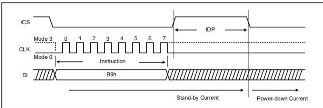
Figure 26a. Deep Power-down Instruction (SPI Mode)
