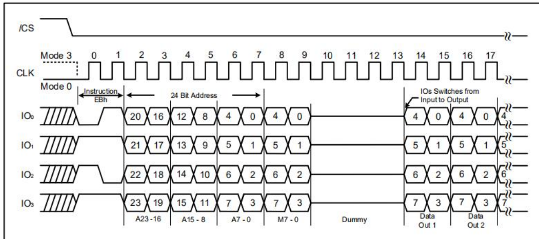
Figure 17d. Fast Read Quad I/O Instruction (Initial instruction or previous M7-0 ≠ Axxh, QPI mode, 108MHz)
