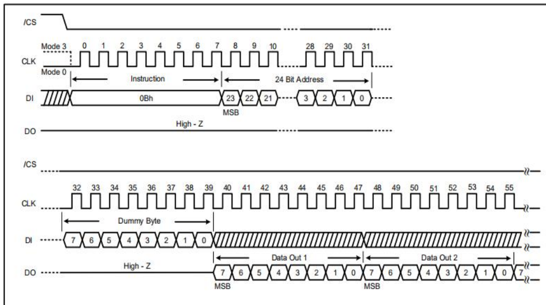
Figure 13a. Fast Read Instruction (SPI Mode)
