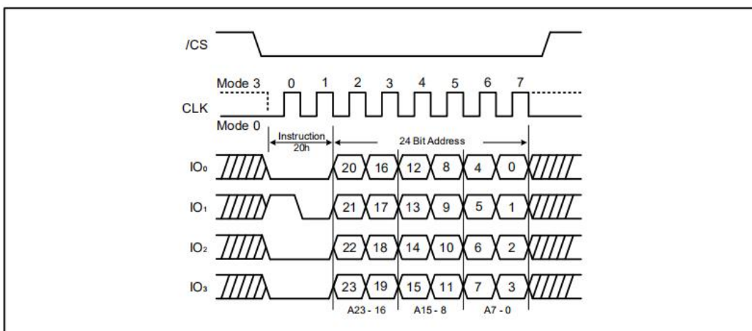
Figure 20b. Sector Erase Instruction (QPI Mode)
