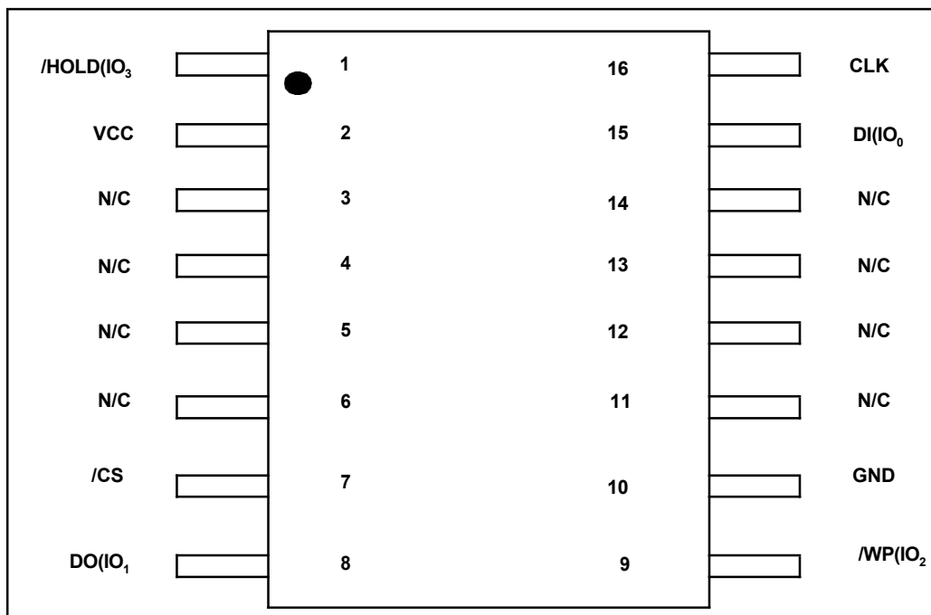
Figure 1c. Pin Assignments, 16-pin SOP 300-mil
