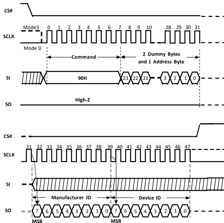
Figure-64. Read Electronic Manufacturer ID & Device ID Sequence Diagram (QPI)
