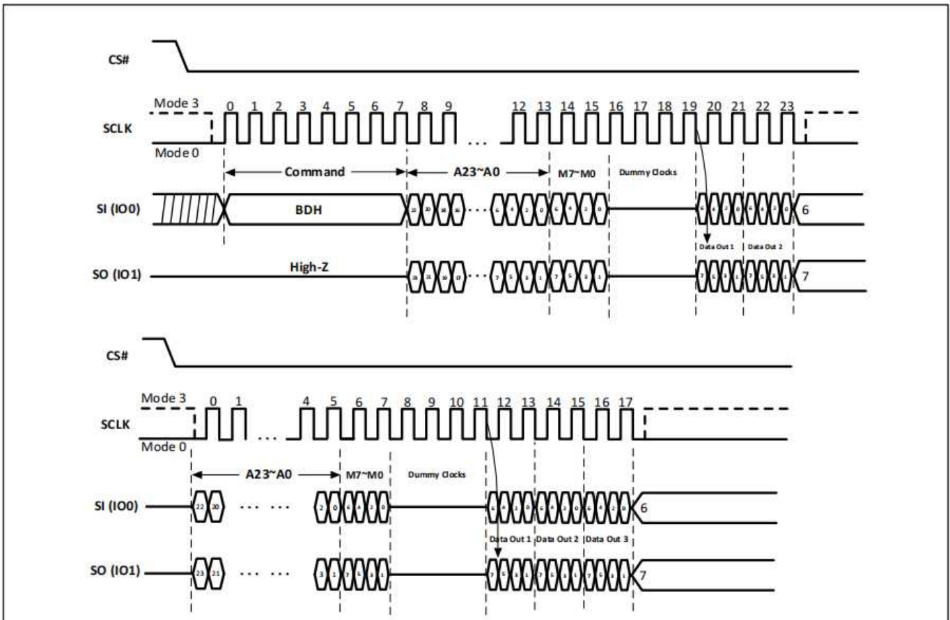
Figure-26. DTR Fast Read Dual I/O with “Continuous Read Mode” Sequence Diagram (M5-4 = (1,0))
