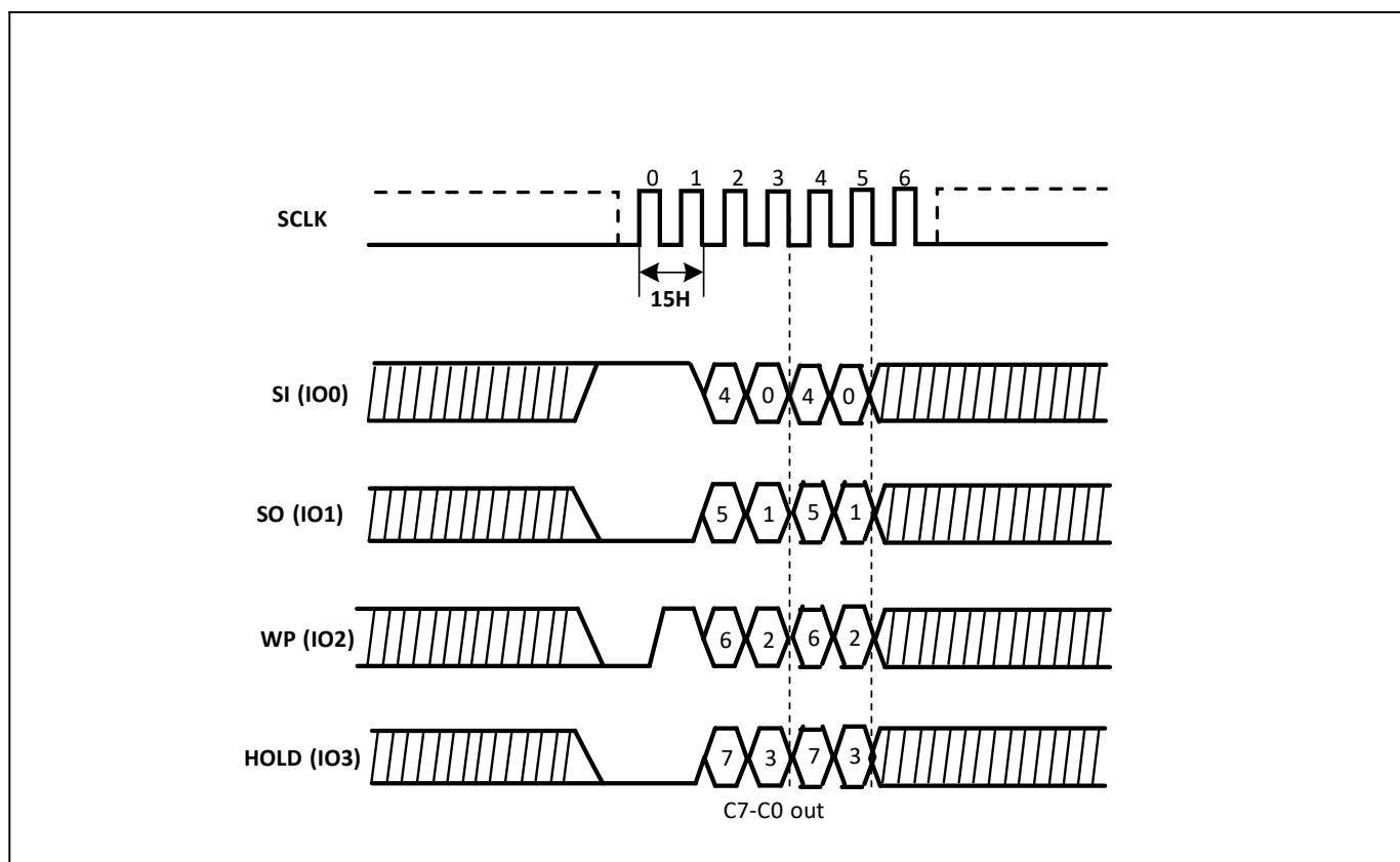
Figure-12. Read Configure Register Sequence Diagram (QPI)
