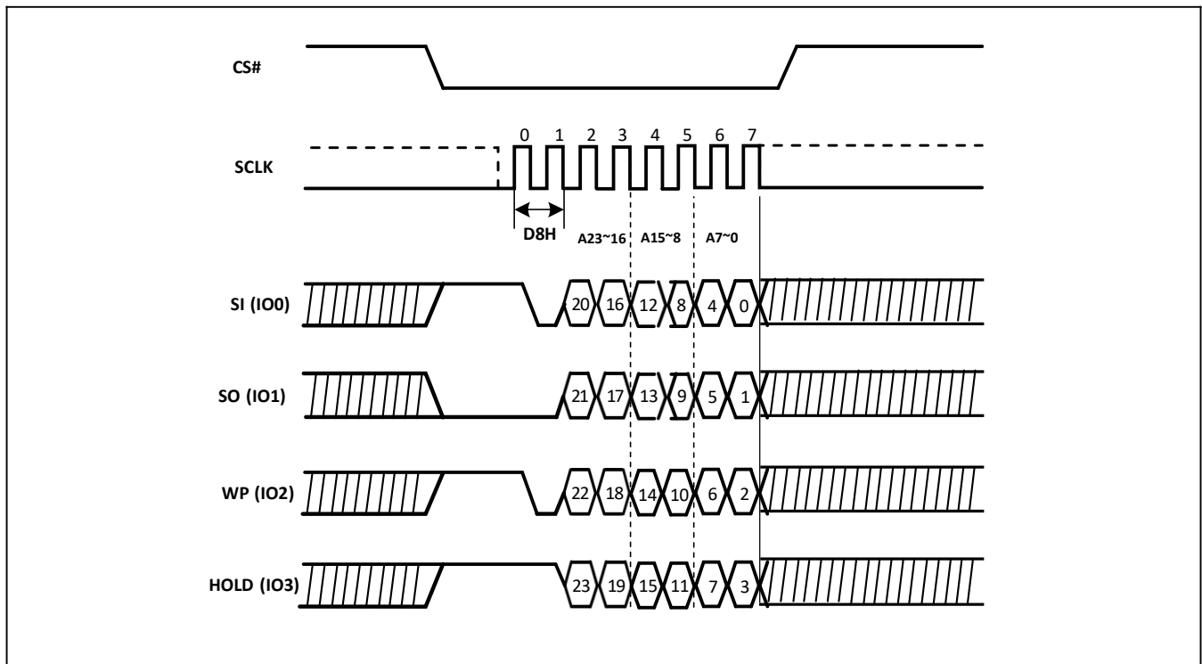
Figure-45. Block Erase Sequence Diagram (QPI)
