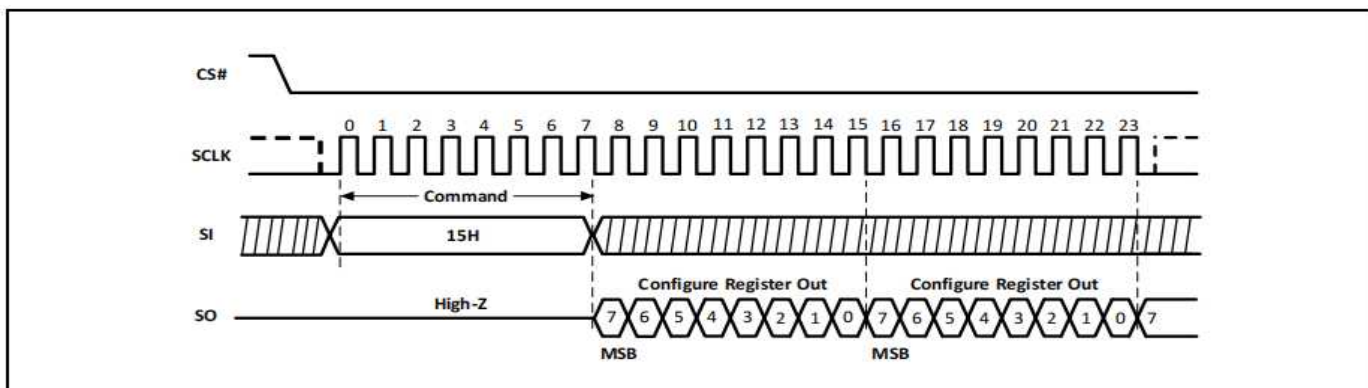
Figure-11. Read Configure Register Sequence Diagram
