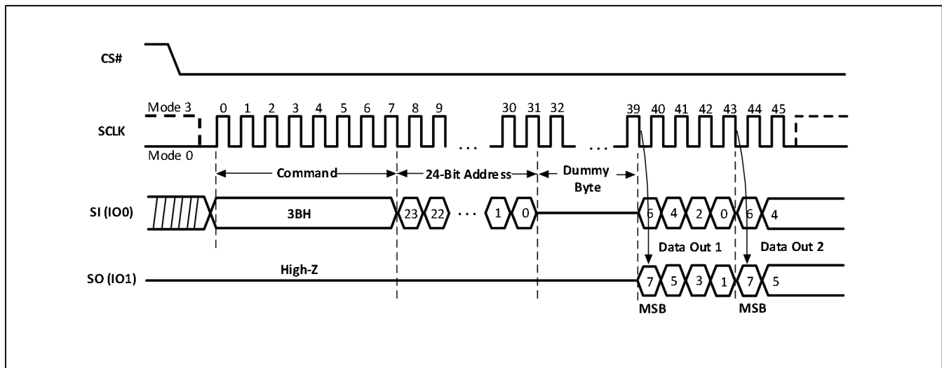
Figure-9. Dual Output Fast Read Sequence Diagram
