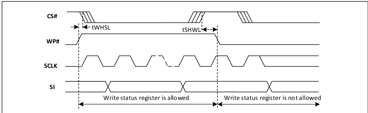
Figure-33. WP Timing
