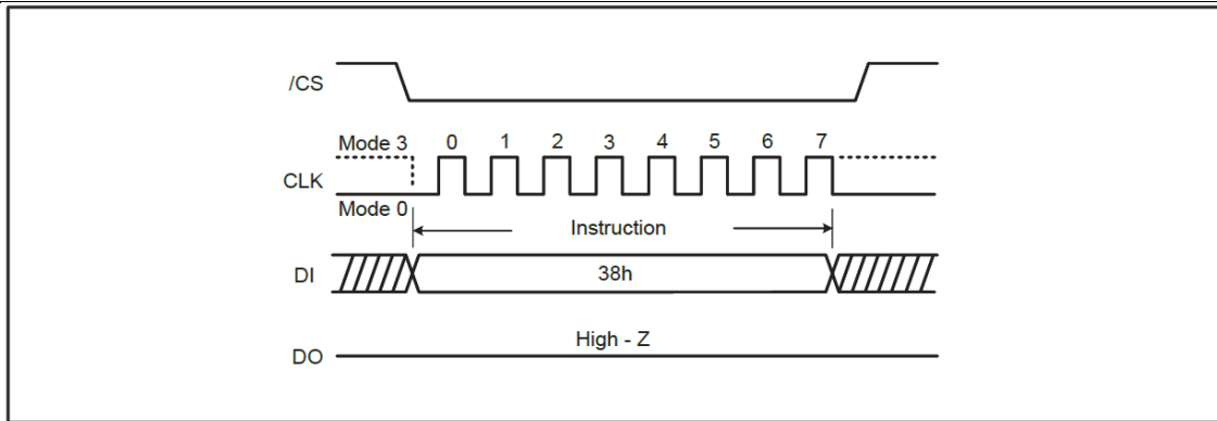
Figure 35, Enable QPI instruction
