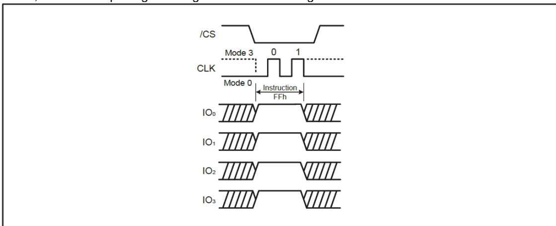
Figure 36. Disable QPI instruction for QPI mode
