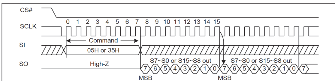
Figure 10, Read Status Register Instruction Sequence Diagram
