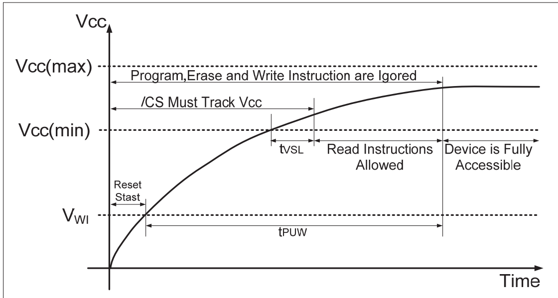
Figure 34, Power-up Timing
