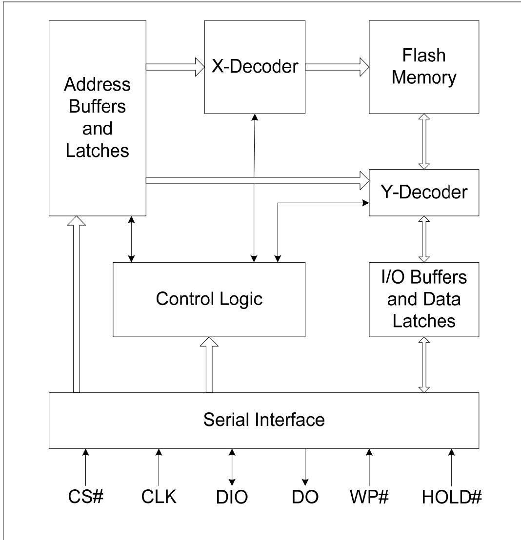
Figure 2, Block Diagram
