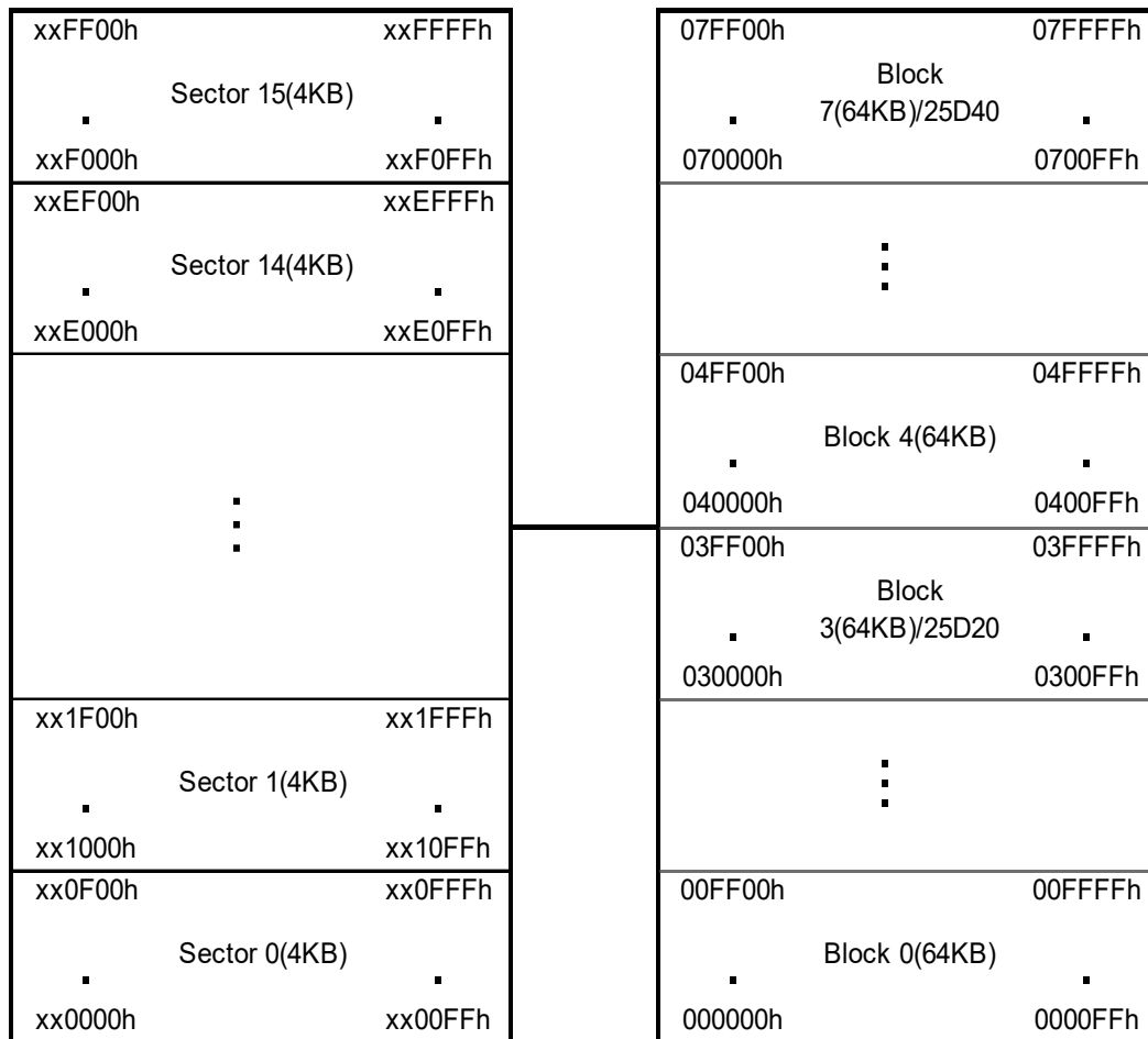
Figure 4, Memory Organization
